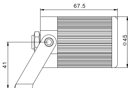
1 mounting hole Ø 7mm
