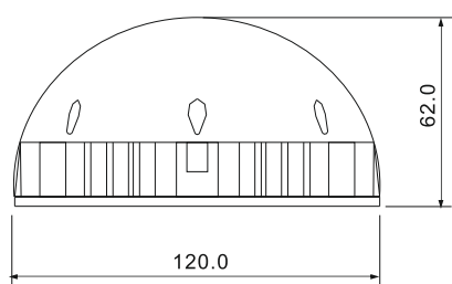
4 mounting holes Ø 5mm, distance 105mm
