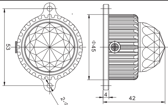
2 mounting holes \varnothing=3,5\text{mm} , distance: 53mm
