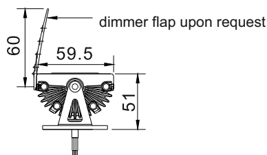
4 mounting holes \varnothing=8.0\text{mm}
