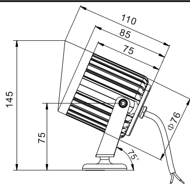
1 mounting hole Ø 7mm
