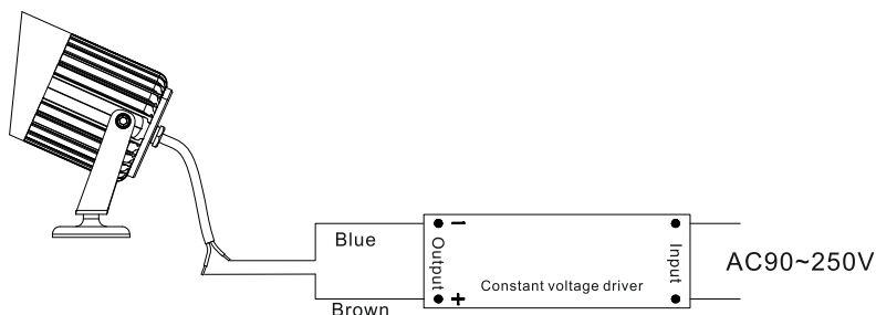
Wiring diagram
